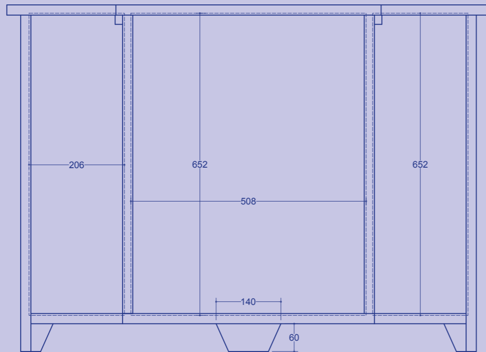
Rear elevation 1 : 8
